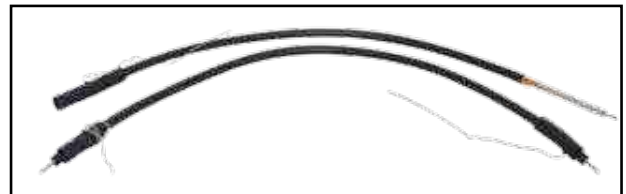
Primary plug and receptacle kit for unscreened cable
