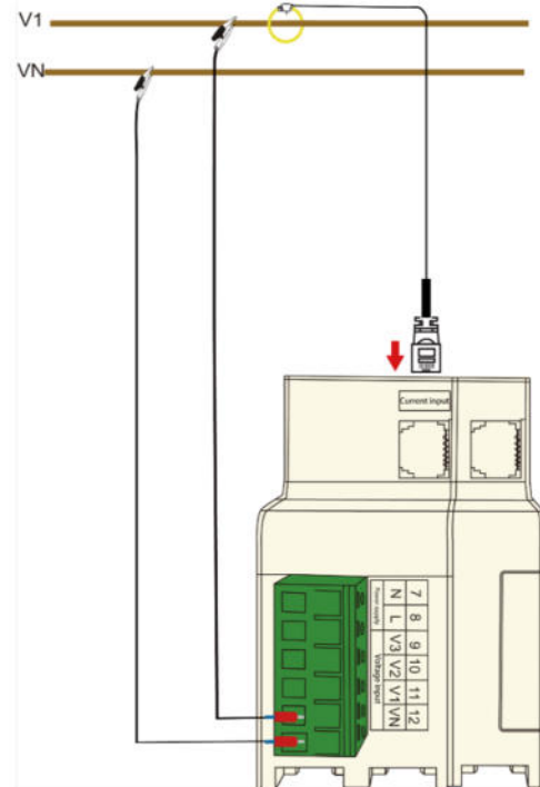
One phase and two-wire
