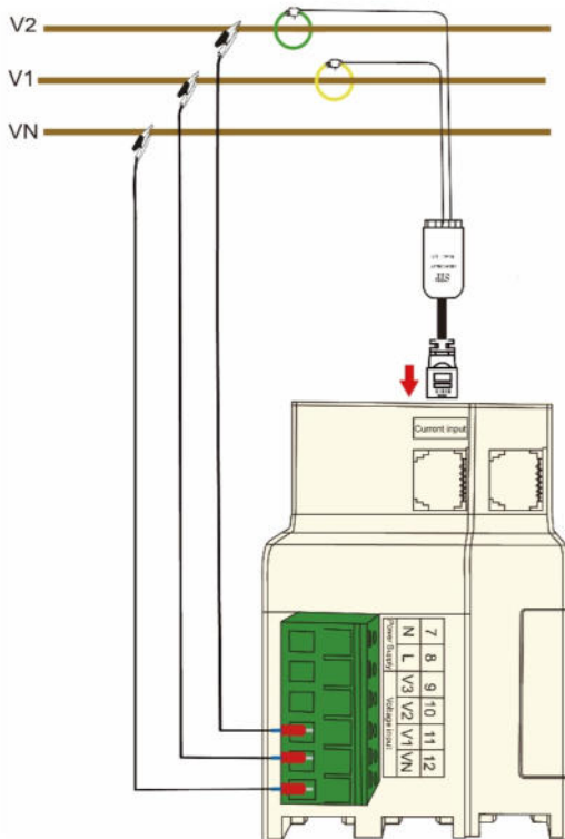
One-phase three-wire
