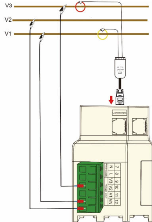
Three-phase three-wire 2CT
