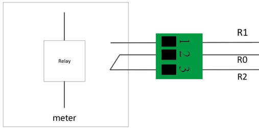
Relay output connection diagram
