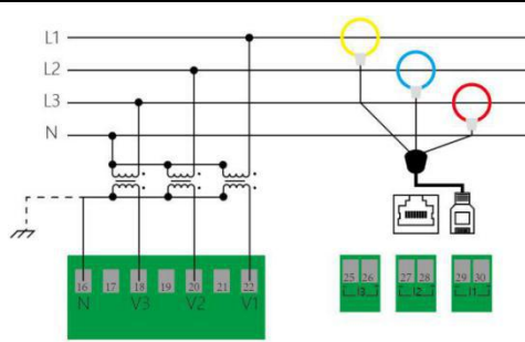
3PH4W(with PT) wiring diagram
